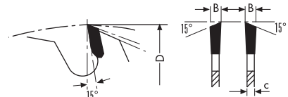
Grooving cutter for "Lamello®"
